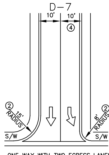
ONE WAY WITH TWO EGRESS LANES (SEE MAG DTL 251)
