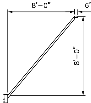
SINGLE ARM
