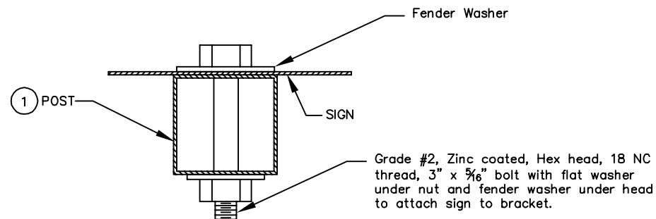
DETAIL A SIGN MOUNTING
