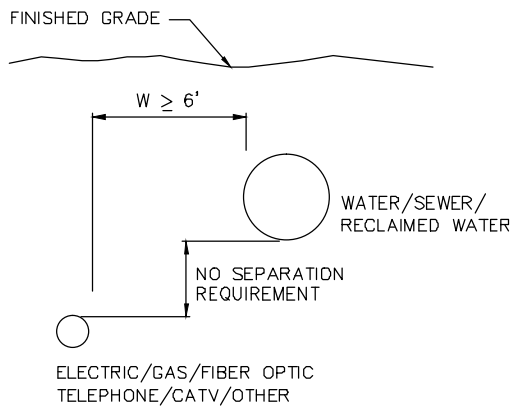
6'+ SEPARATION
