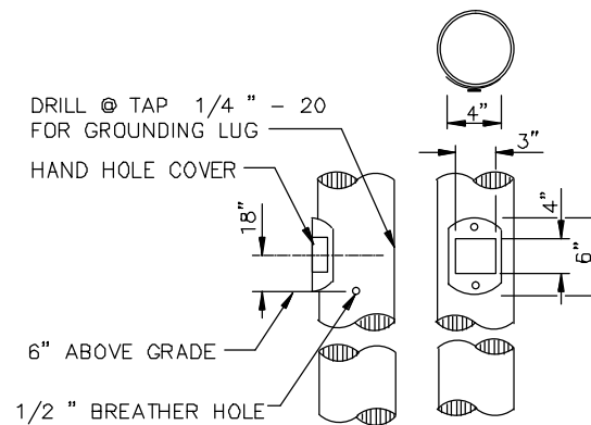
PENETRATIONS
