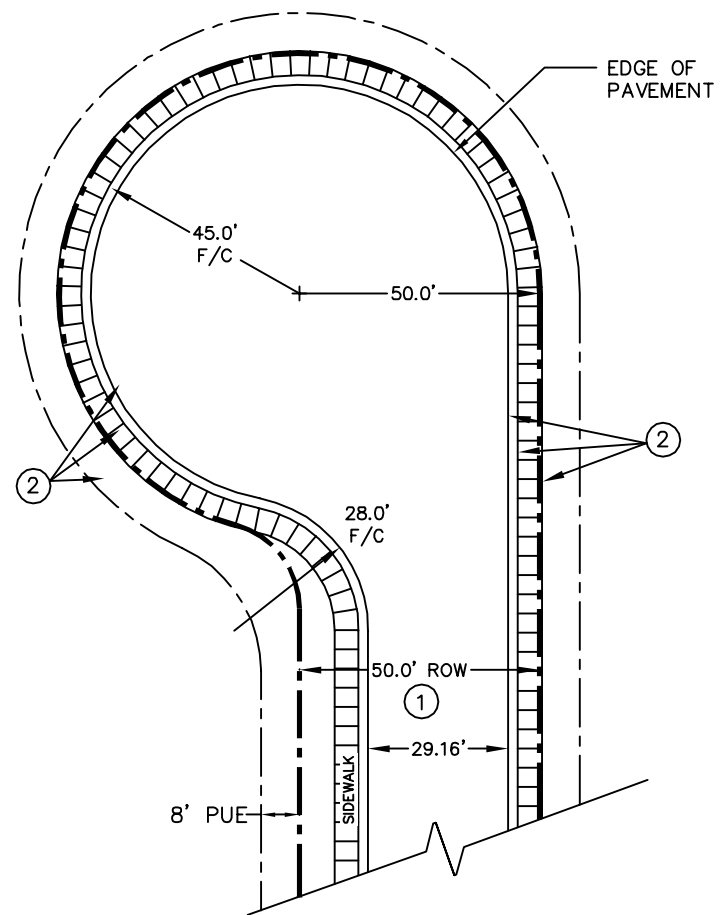
MODIFIED CUL-DE-SAC
