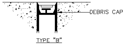
TYPE "B"
