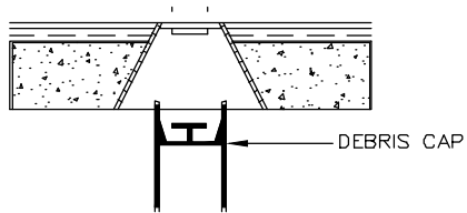
TYPE "A"
