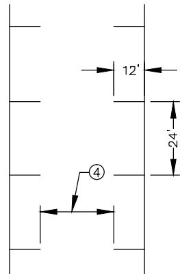
PARALLEL PARKING
