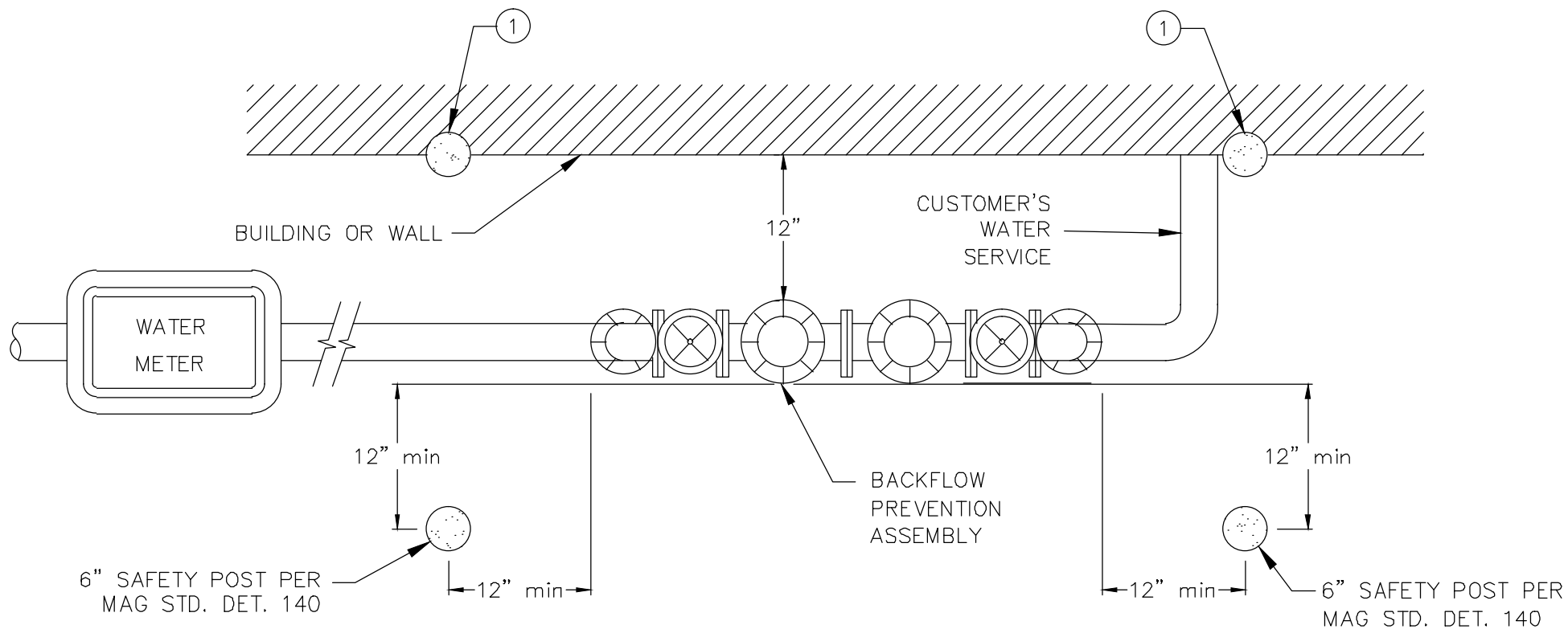
PLAN VIEW
