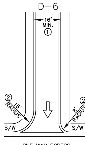
ONE WAY EGRESS (SEE MAG DTL 251)
