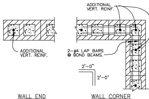
WALL END
