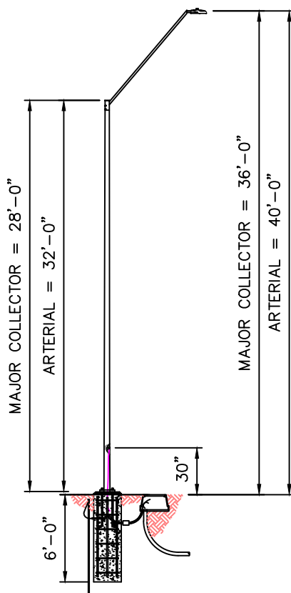
MAJOR COLLECTOR/ARTERIAL
