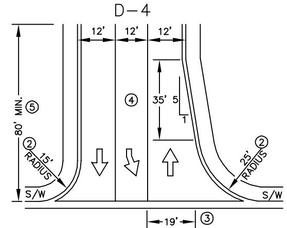
TWO WAY WITH TWO EGRESS LANES (SEE MAG DTL 251)
