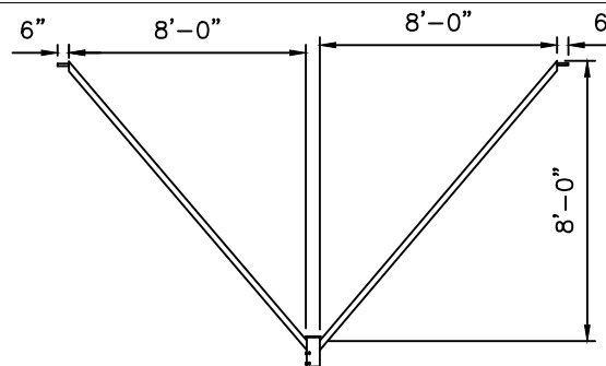
DOUBLE ARM
