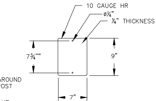
HANDHOLE COVER DETAIL
