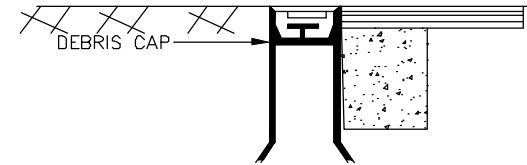
TYPE "C"
