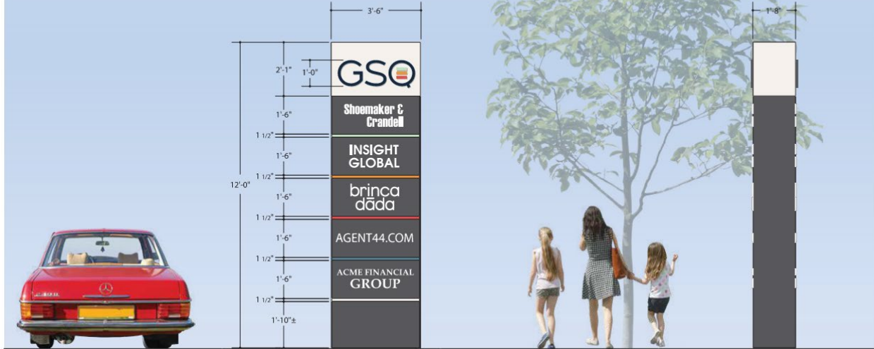
A-4: SECONDARY IDENTITY | TENANT MONUMENT Scale: 3/8"=1'-0"
