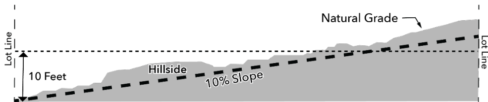
Figure 4.7.2A - Hillside Identification
