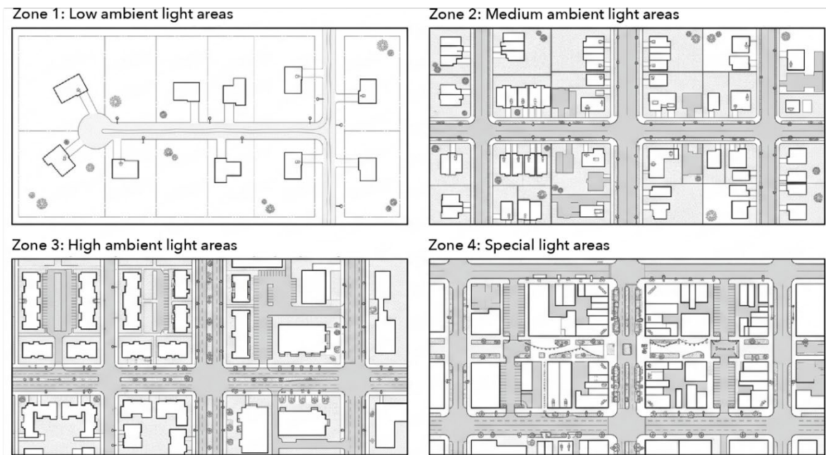
Figure 4.5.3A - Lighting Zones
