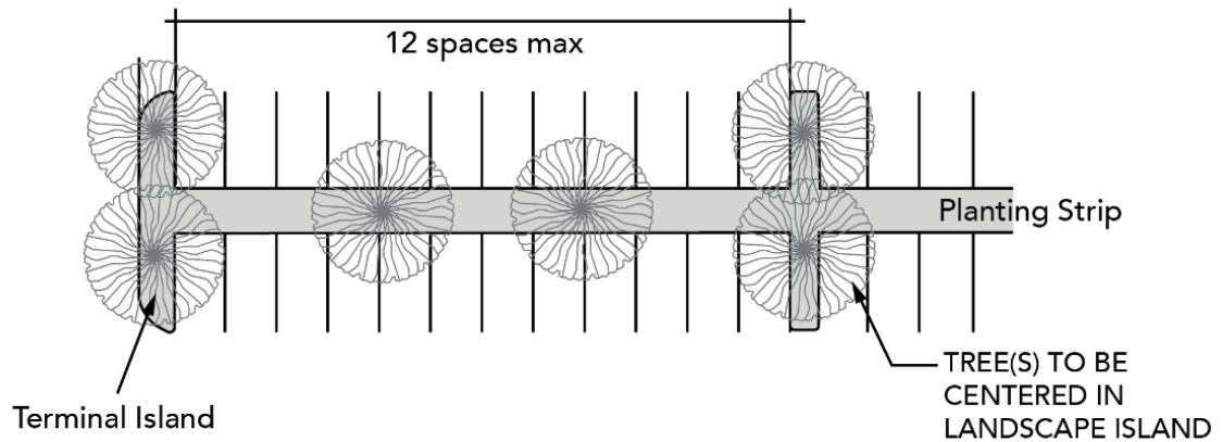
Figure 4.2.4A - Parking Area Landscaping
