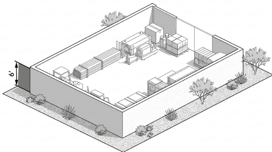
Figure 4.3.1A - Outdoor Storage Screening
