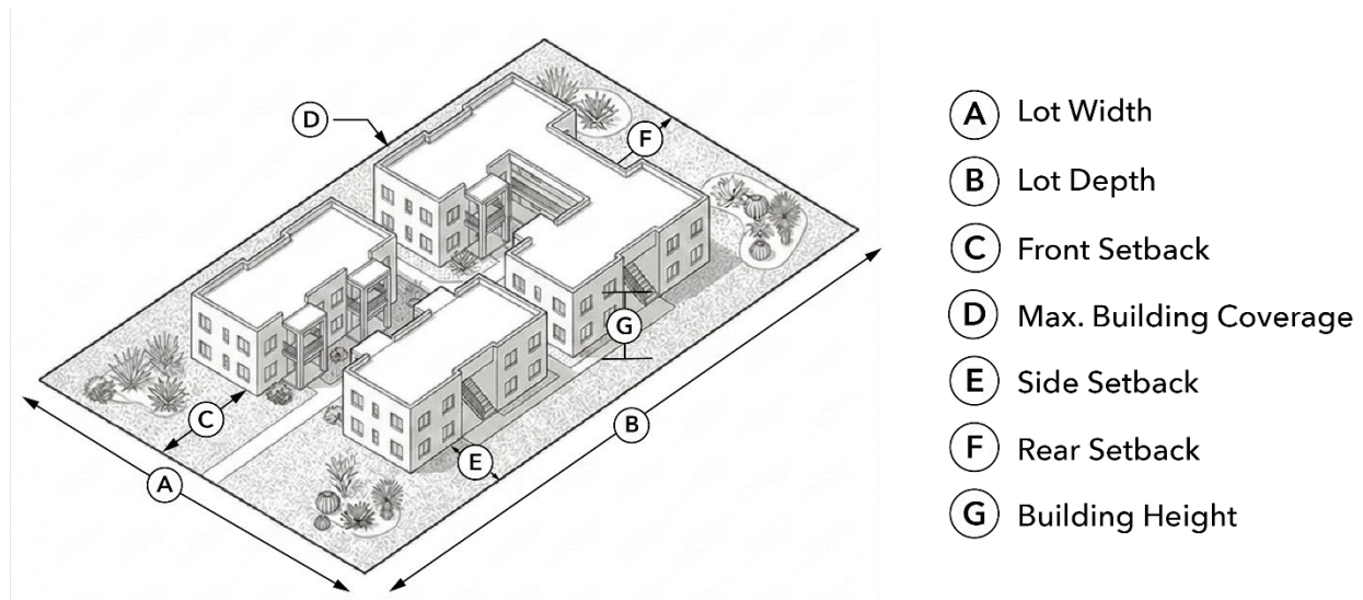
Figure 2.2.4A – Multi-Family Residential Setbacks
